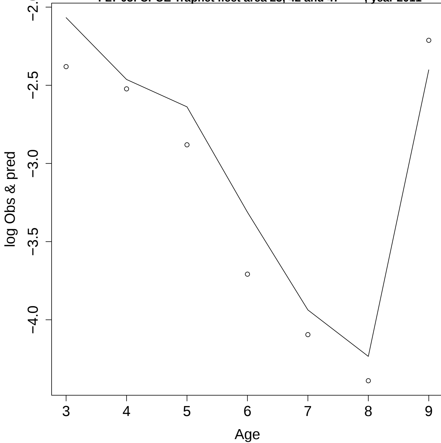
FLT 03: CPUE Trapnet fleet area 23, 42 and 47 , year 2011
