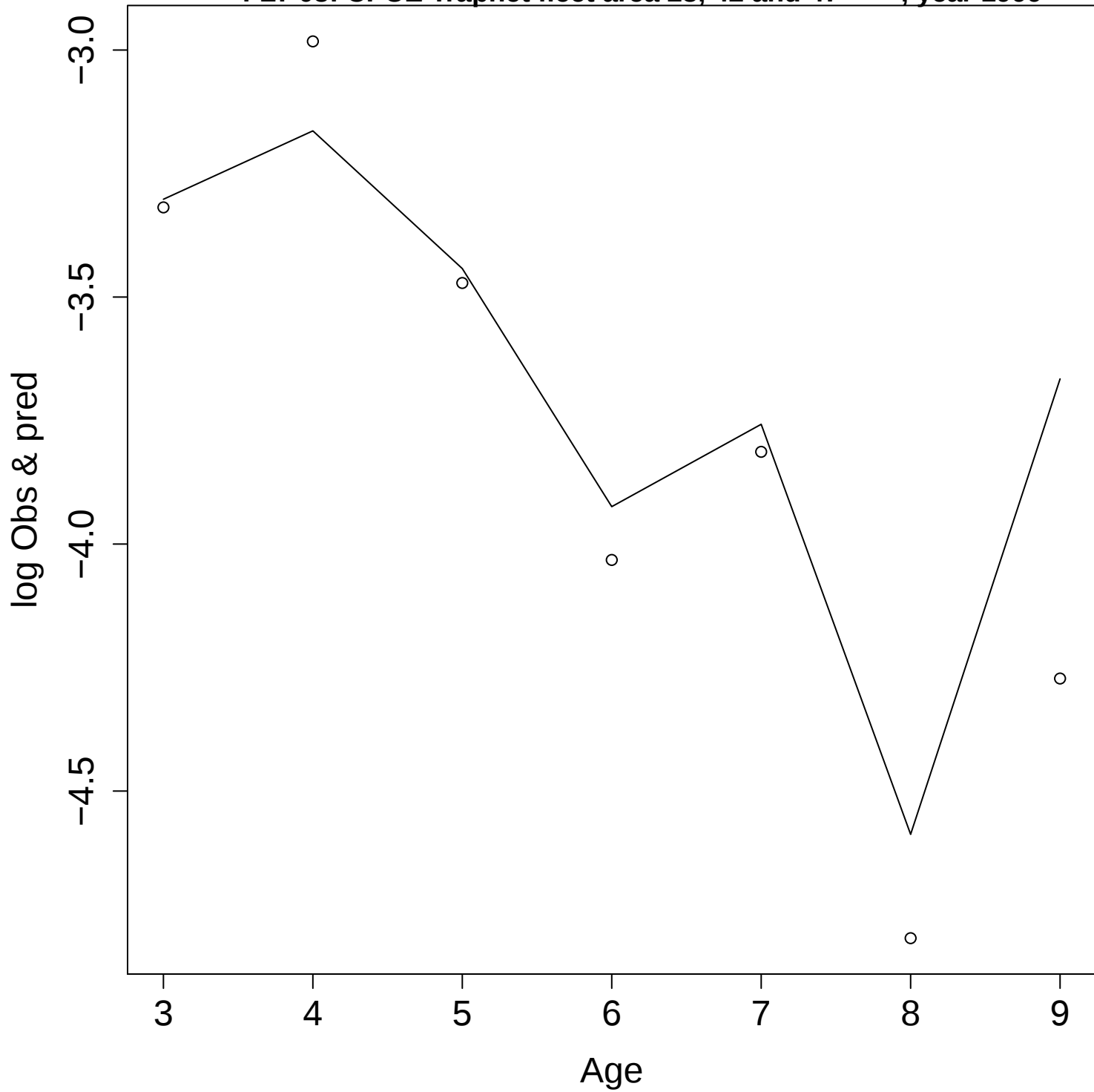
FLT 03: CPUE Trapnet fleet area 23, 42 and 47 , year 1999
