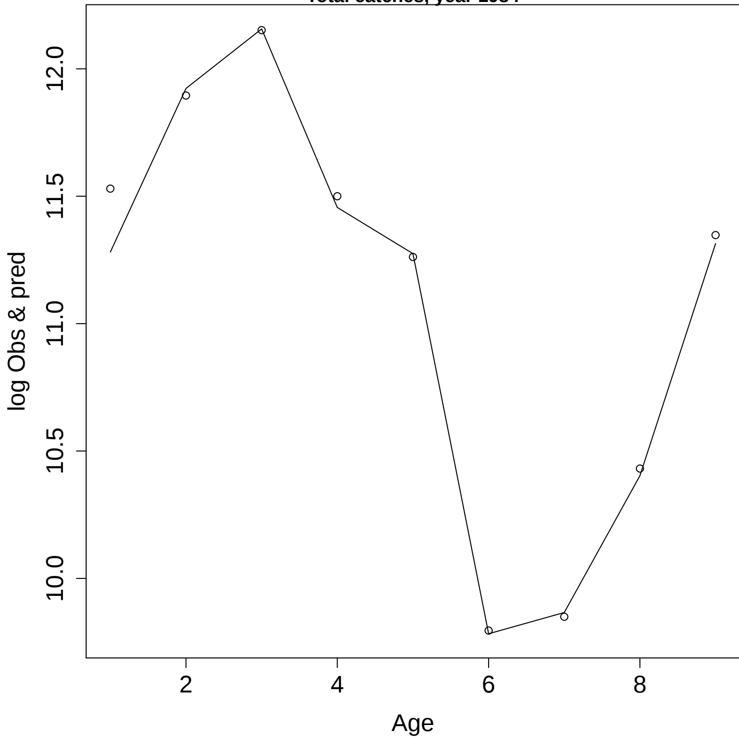
Total catches, year 1984
