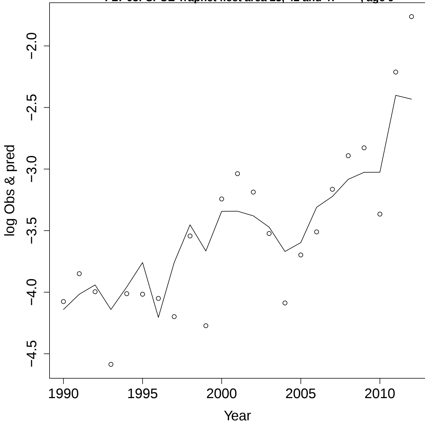
FLT 03: CPUE Trapnet fleet area 23, 42 and 47 , age 9
