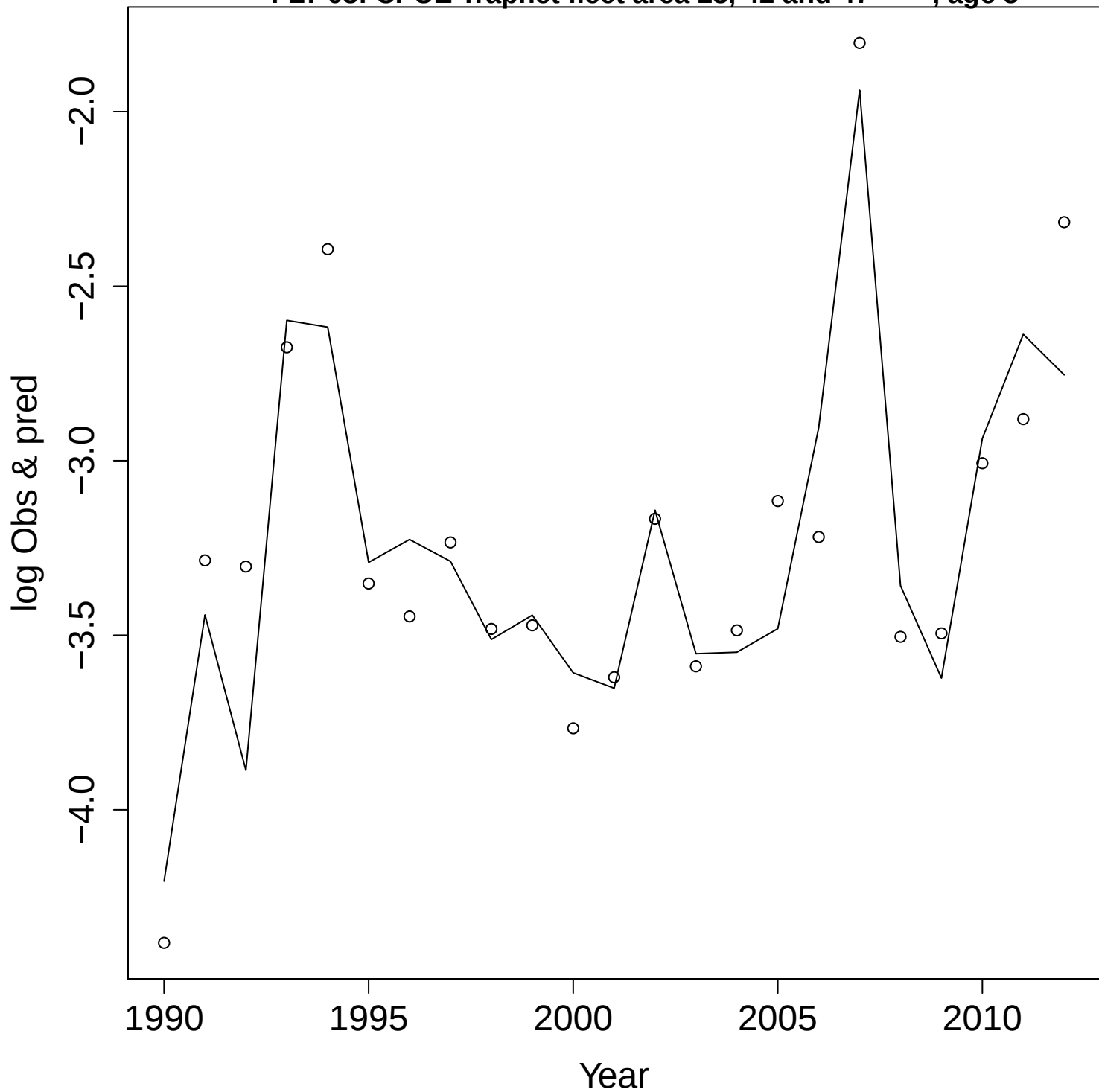
FLT 03: CPUE Trapnet fleet area 23, 42 and 47 , age 5
