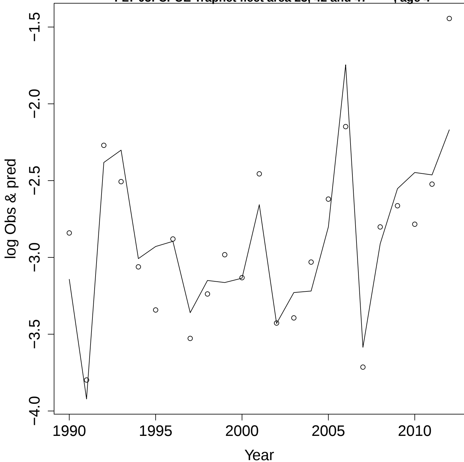
FLT 03: CPUE Trapnet fleet area 23, 42 and 47 , age 4
