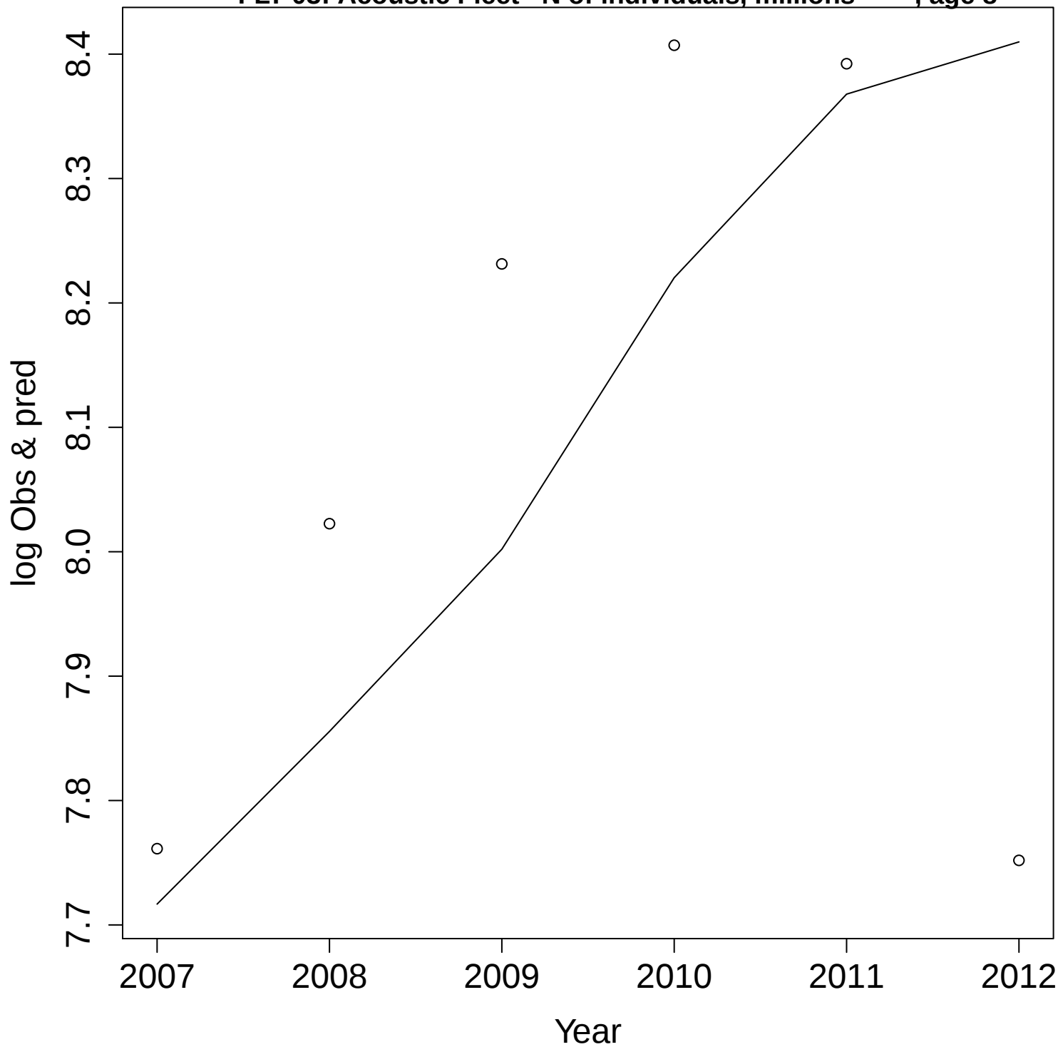
FLT 03: Acoustic Fleet N of individuals, millions, age 8
